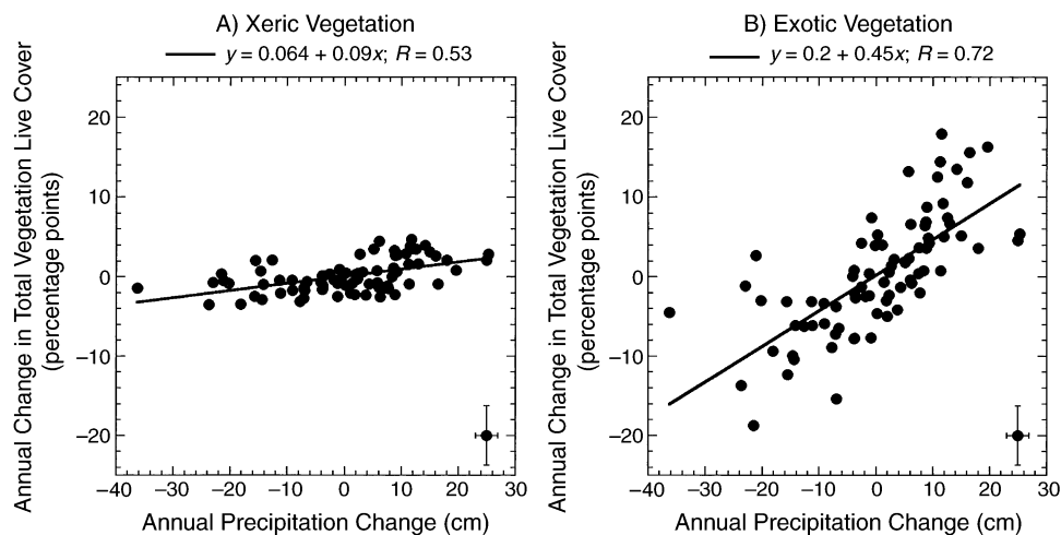
FIG. 7. Comparison of Landsat derived annual change in percent live cover and annual change in precipitation for (A) xeric plant communities and (B) parcels dominated by exotic annuals for the years 1990–1996. Correlations were significant for both community types ( P < 0.01 ); error estimates are presented in the lower right of each graph and were derived as in Fig. 6.
