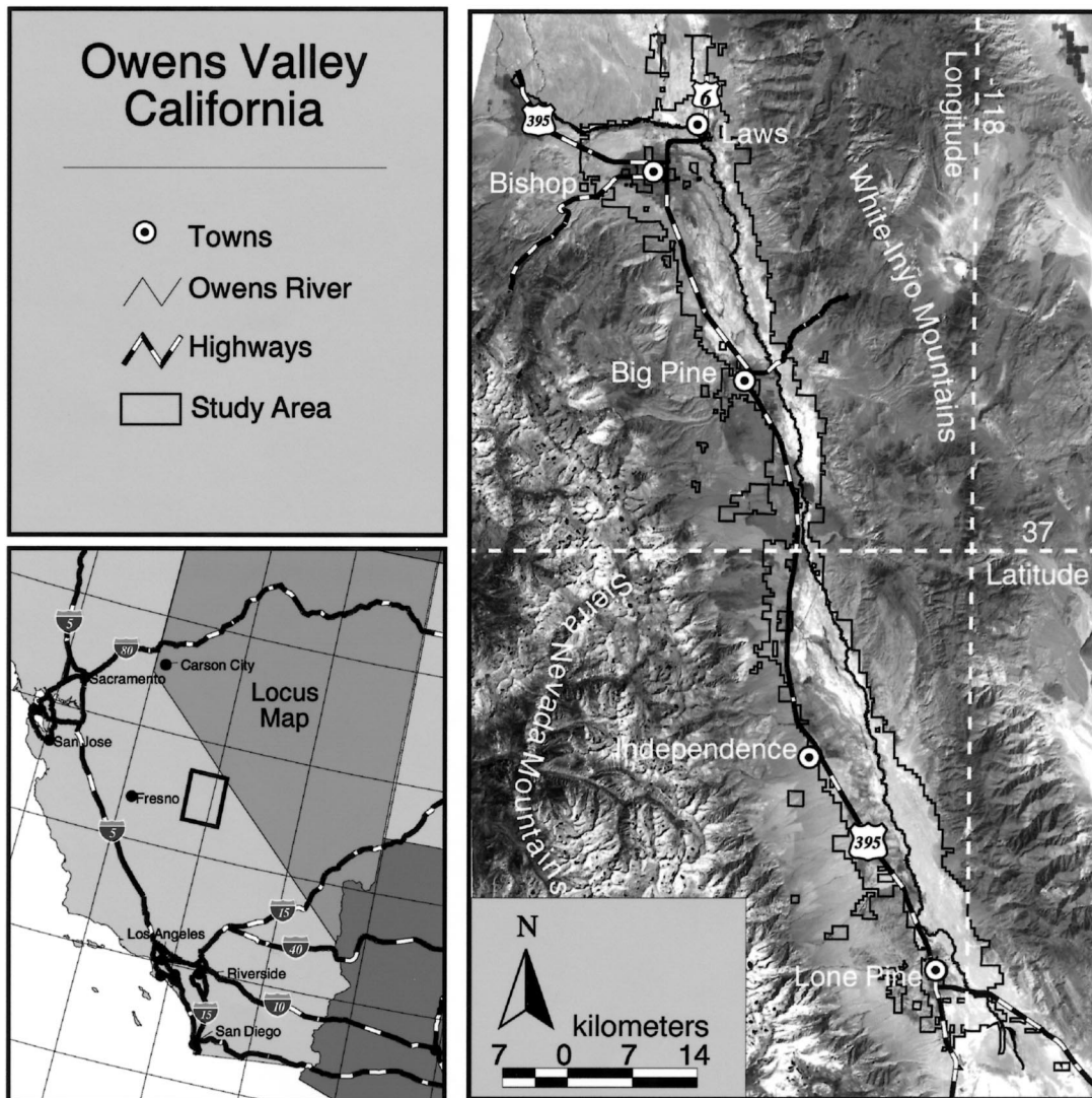
FIG. 1. Location of Owens Valley, California, and map of study area and major features.
