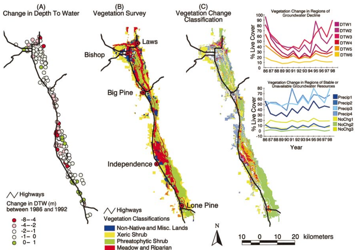
FIG. 4. Maps showing the spatial extents of (A) the change in depth to water recorded by 171 piezometers between 1986 and 1992; (B) the plant community distribution mapped by LADWP during a 1984–1987 inventory; and (C) the distribution of 13 vegetation response classes resulting from spectral mixture analysis (SMA) of Landsat TM data. Riparian communities, which represent a relatively small area at this scale, have been added to meadow communities in (B). The two graphs in the upper right show the 1986–1998 annual average percent live cover for each change class in (C). DTW, Precip, and NoChg designate change classes representing depth to water dependent changes, precipitation dependent changes, and static vegetation conditions, respectively (see Results: Linking environmental drivers ).
