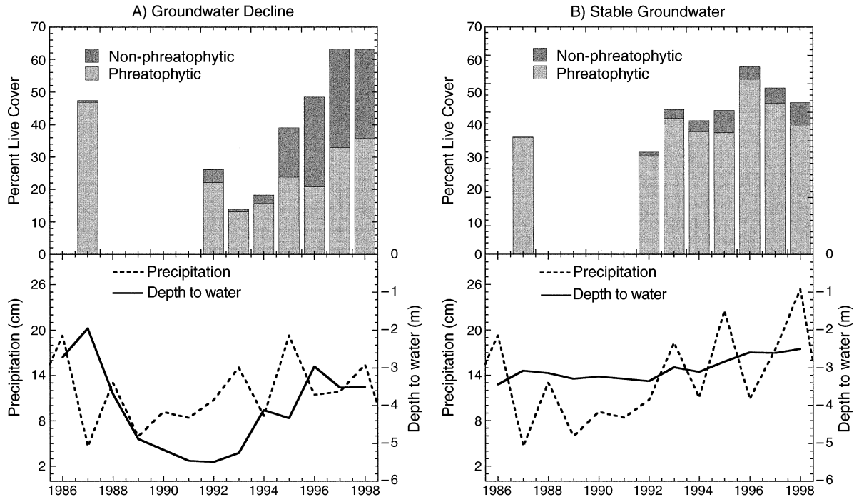
FIG. 5. Comparison of field-measured vegetation conditions, depth-to-groundwater, and annual precipitation in two meadow parcels monitored by Inyo County: (A) parcel LAW107, which exhibited a decline in water table, showed a decline in phreatophytic and an increase in nonphreatophytic (typically exotic annual) species; (B) parcel PLC121, which exhibited stable groundwater and vegetation conditions, including a constant relative proportion of phreatophytic and nonphreatophytic species.
