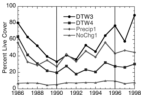
FIG. 8. Three primary modes of response were detected in Owens Valley over the 13-yr period: no change (NoChg), changes attributable to groundwater fluctuations (DTW), and changes amplified with respect to precipitation (Precip). Within these general categories, 13 classes were distinguished; examples of four are shown. For each of the three categories, unique features of the respective response pattern were used to separate individual change classes. For DTW, the linear decline in live cover between 1986 and 1992 was found to be distinct from that exhibited in the other change classes. After 1992, the Precip classes exhibited a response correlated with and amplified with respect to precipitation (Fig. 3). If a class exhibited a response characteristic of both DTW and Precip classes, it was assigned DTW; however a response amplified with respect to precipitation indicates the presence of exotic annuals in most cases.
