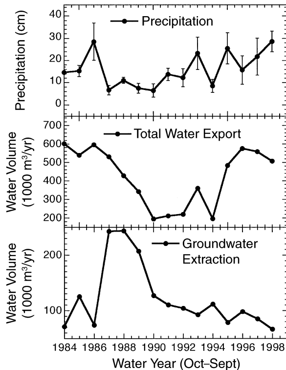
FIG. 3. Recent timeline for Owens Valley showing average annual precipitation (six gauges), total water export, and total water extracted from groundwater resources. A pronounced drought between 1987 and 1992 is exhibited explicitly or implicitly in all three quantities. As an indication of the scarcity of water between 1987 and 1992, groundwater extraction volumes nearly equaled total water export from the valley at this time. Precipitation error bars show one standard deviation from the mean.
